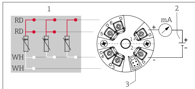
3 Terminal assignment of head transmitter
