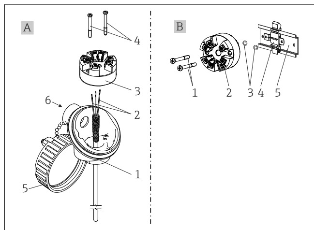
2 Head transmitter mounting
